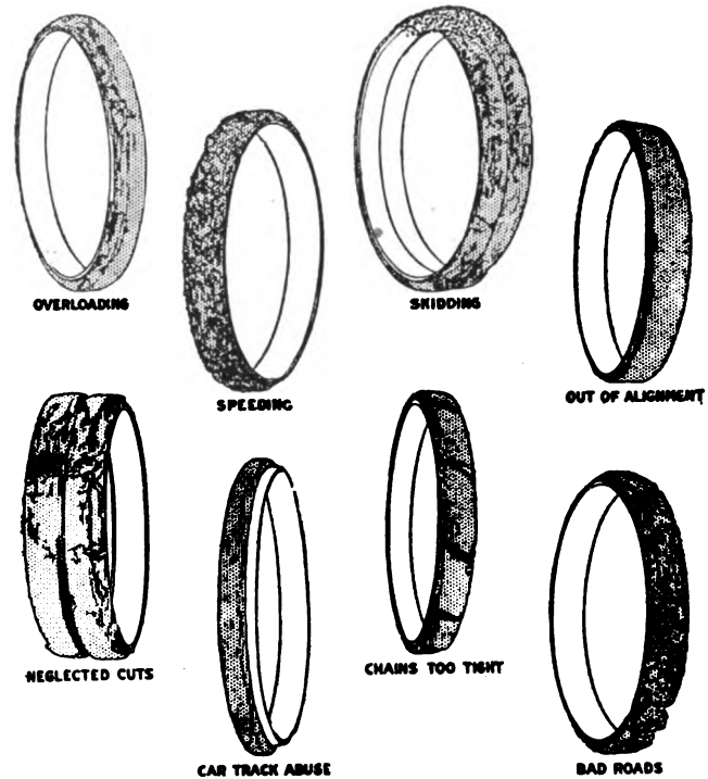
Illustrating the results of various forms of truck tire abuse. These drawings may be used as a key to ascertain just what is doing the damage and to rectify it
